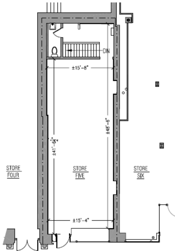
COLUMBUS AVENUE ① PLAN - GROUND FLOOR LEVEL NORTH
