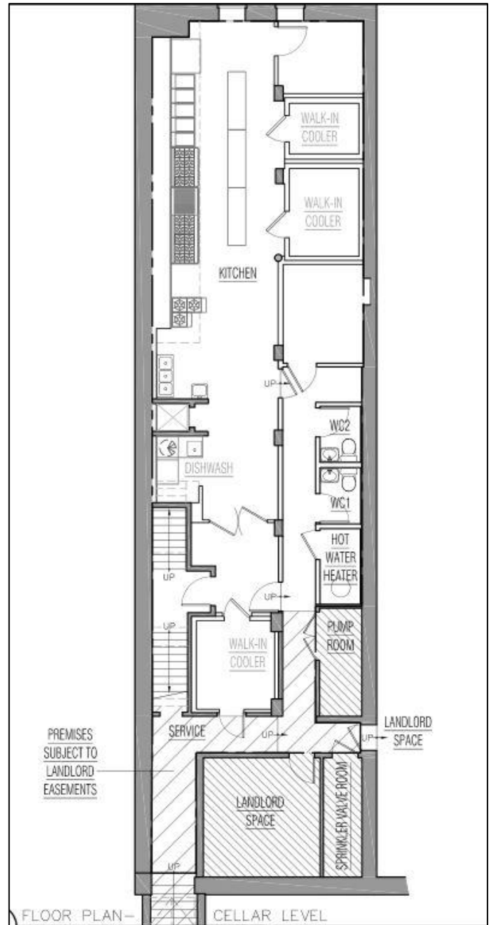
Cellar Plan
