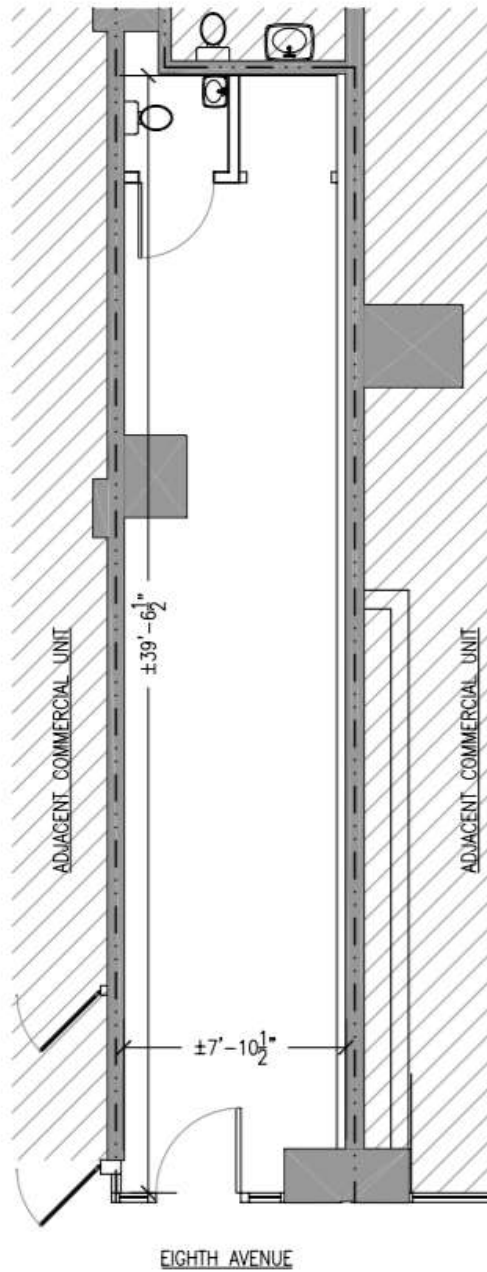
1 FLOOR PLAN - STORE 4 - GROUND FLOOR LEVEL SCALE: 3/16" = 1'-0"
